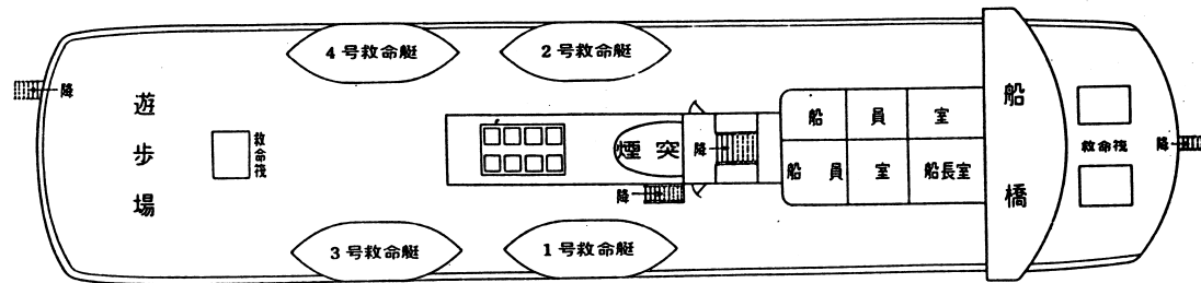
端艇甲板 BOAT DECK
